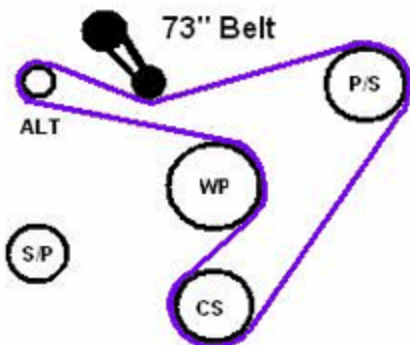
Bypassing the smog pump and using the Ford Racing M-8511-A50 A/C Eliminator
