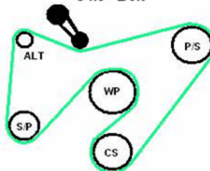
Factory setup without A/C or using Ford Racing M-8511-A50
