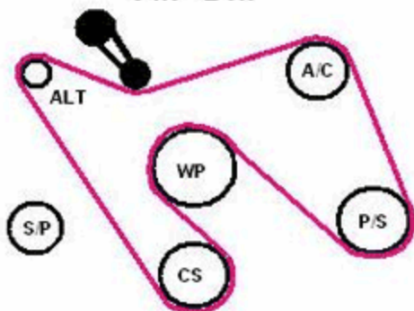
Bypassing the smog pump and using the Ford Racing M-8511-A50 A/C Eliminator
